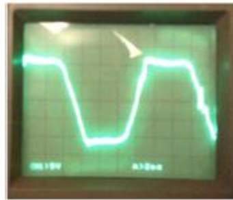
Generator output large load
