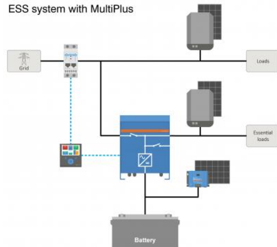
ESS system with MultiPlus
